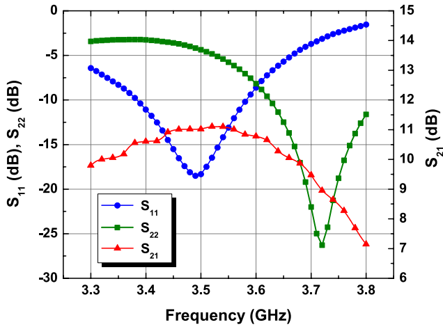
Figure 14 - Typical S_{11} and S_{21}
