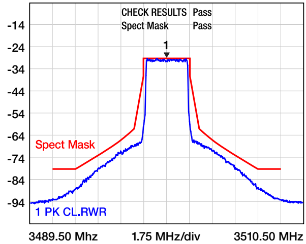
Figure 13 - ETSI Mask Compliance in Nitronex Demonstration Board at 3500MHz and P_{OUT} = 1.5W
