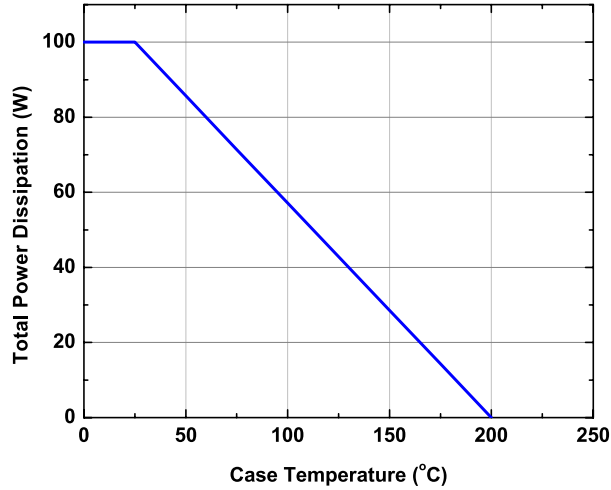
Figure 18 - Power Derating Curve
