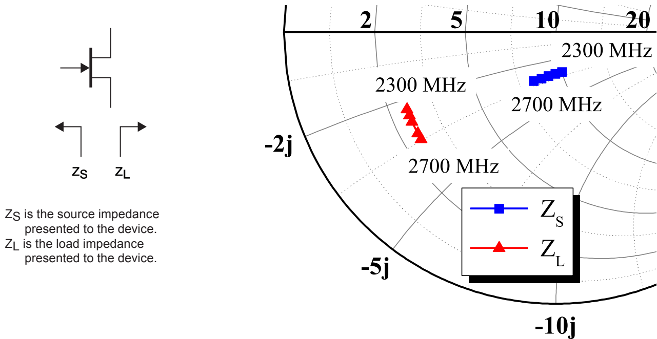
Figure 1 - Optimal Impedances for CW Performance, V_{DS} = 28V , I_{DQ} = 600mA
