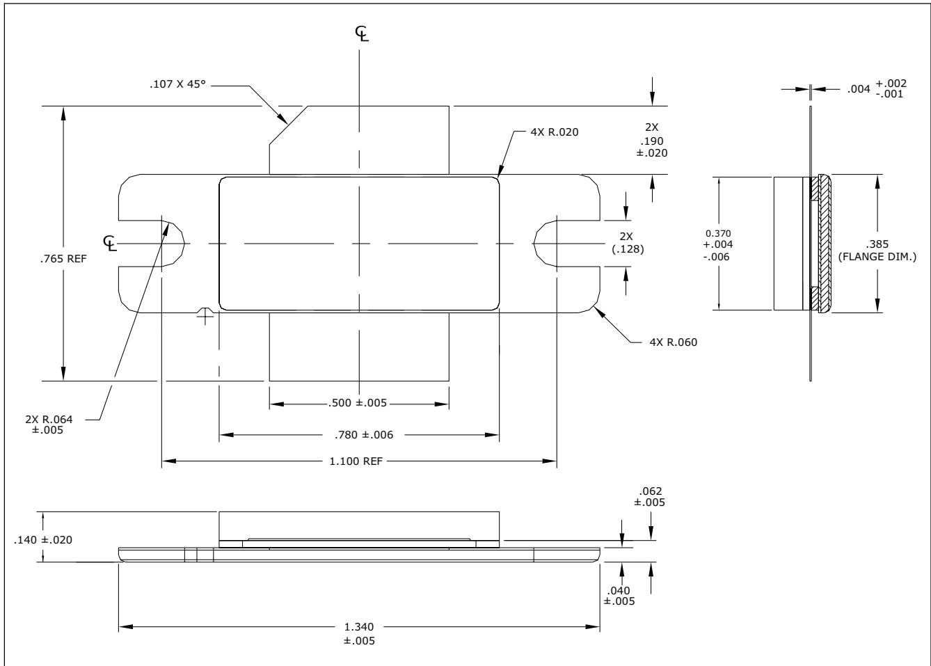
Figure 22 - AC780BC-F2 Package Dimensions and Pinout (all dimensions are in inches)
