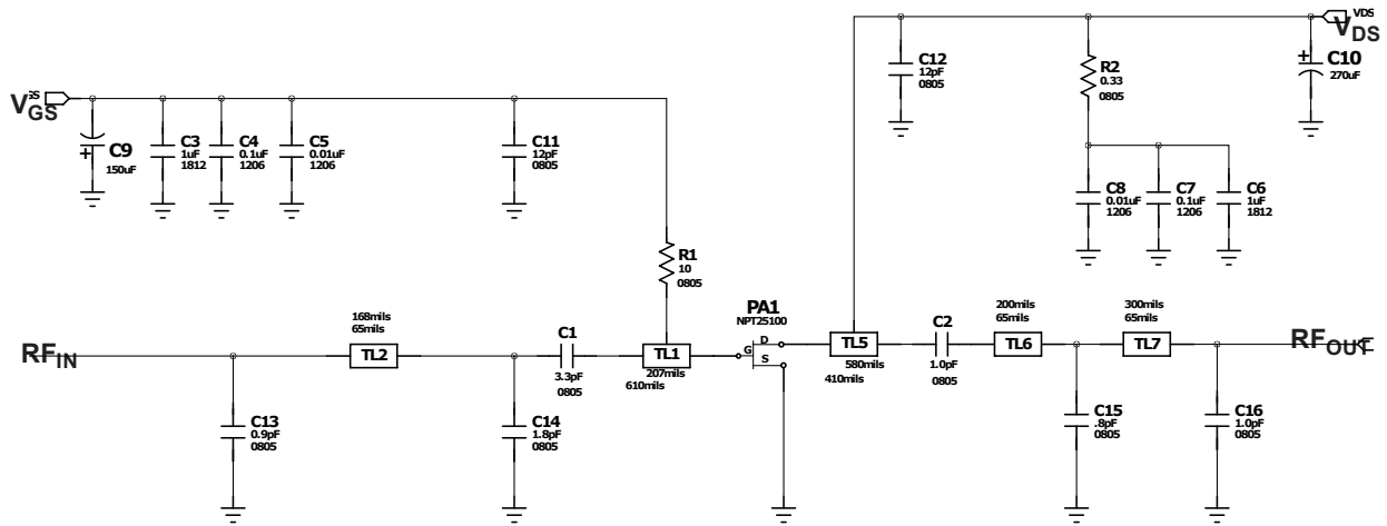
Figure 21 - APP-NPT25100-25 2500MHz Demonstration Board Equivalent Circuit
