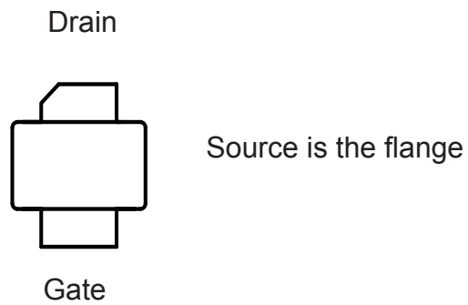
Figure 23 - Terminal Identification
