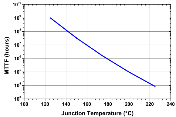
Figure 11 - MTTF of NRF1 Devices as a Function of Junction Temperature
