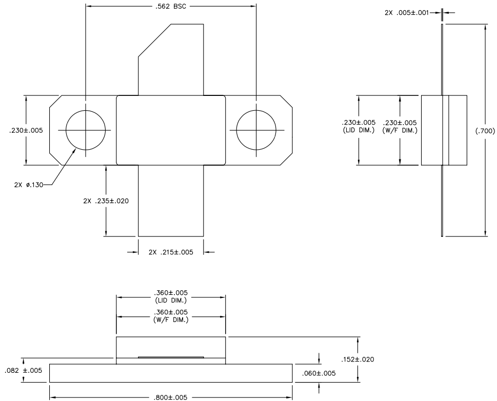
Figure 20 - AC360BC-F2 Package Dimensions and Pinout (all dimensions are in inches)
