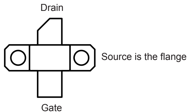
Figure 21 - Terminal Identification
